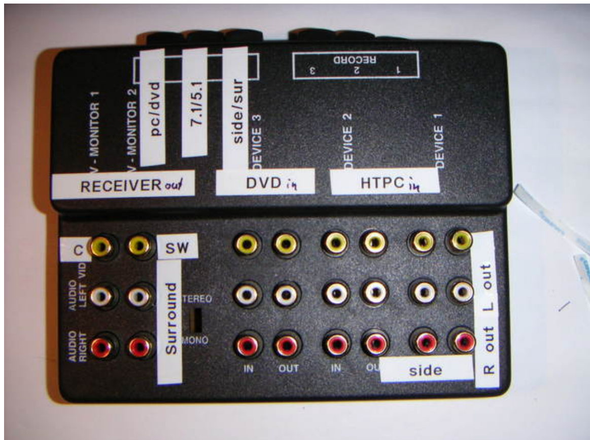
The switch-box, front view
